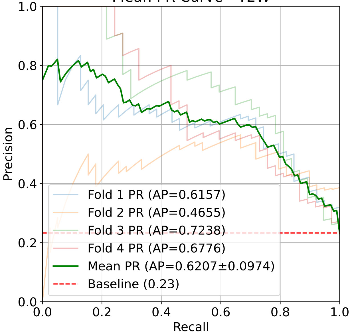
Mean PR Curve - T2W
